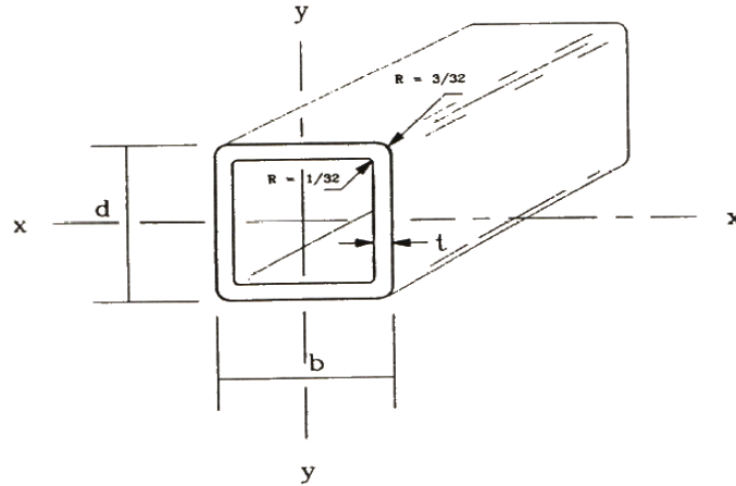
RECTANGULAR TUBE
